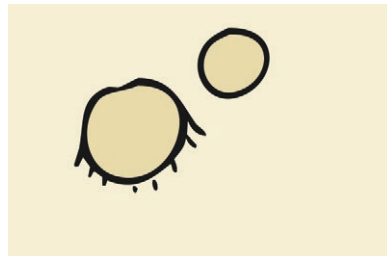
craters
